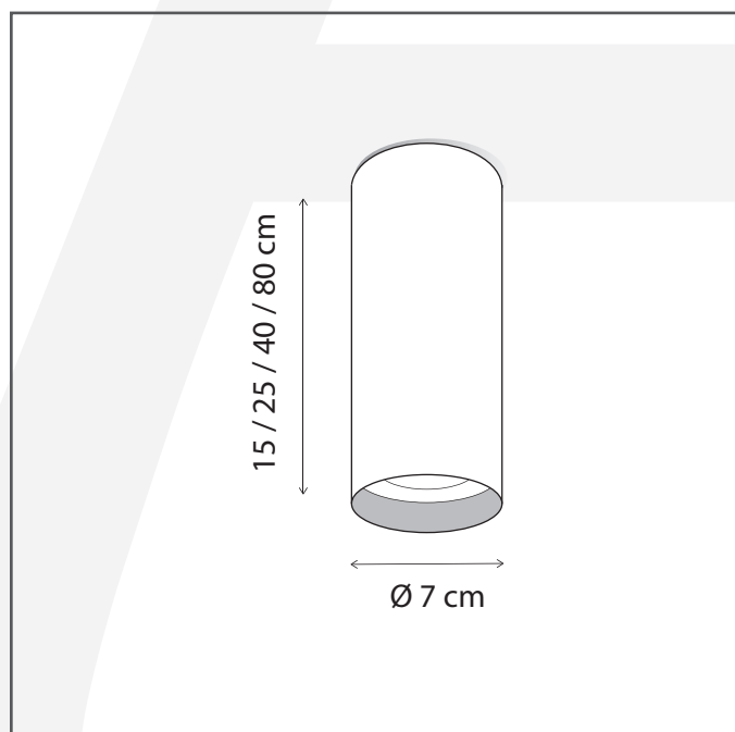
Tubelum ceiling
