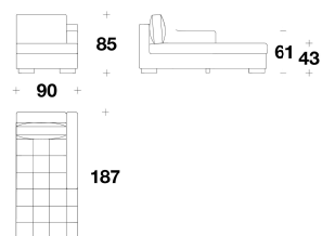
SHT (CLD) - SHT (CLS) CHAISE LONGUE DX O SX / RIGHT OR LEFT CHAISE LONGUE 90x187x85H. - H.SA.61 - H.S.43cm 35 1/3x73 2/3x33 1/3H. - H.SA.24 - H.S.17"
